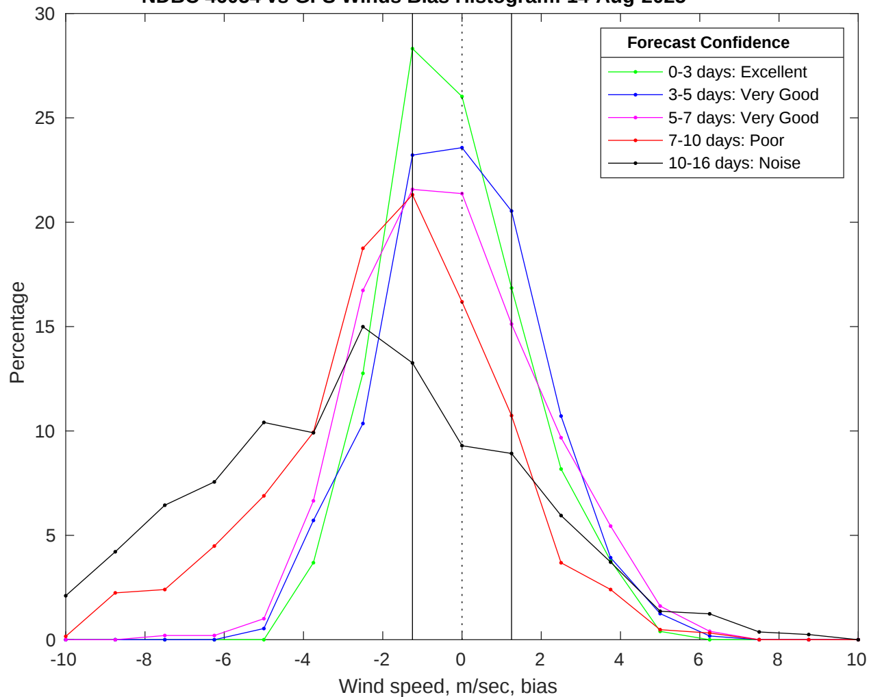
NDBC 46054 vs GFS Winds Bias Histogram: 14-Aug-2025
