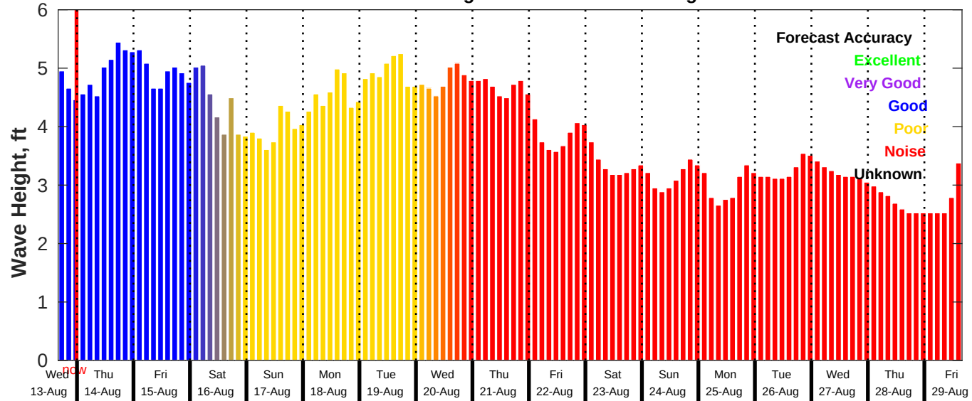
GFS Wave Forecast for NDBC 46054 from 13-Aug-2025 16:00:00 to 29-Aug-2025 16:00:00
