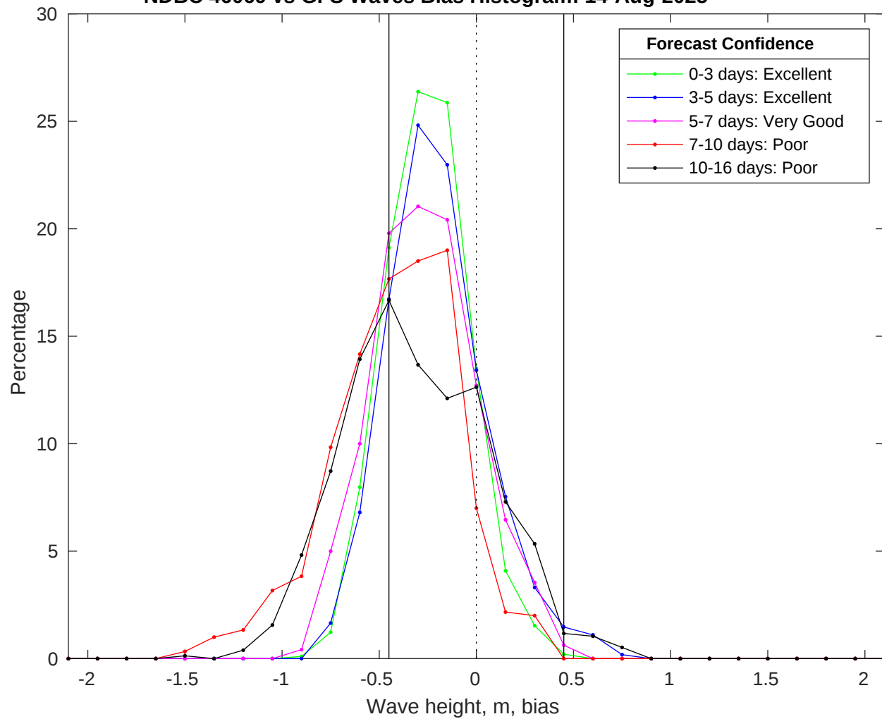
NDBC 46069 vs GFS Waves Bias Histogram: 14-Aug-2025
