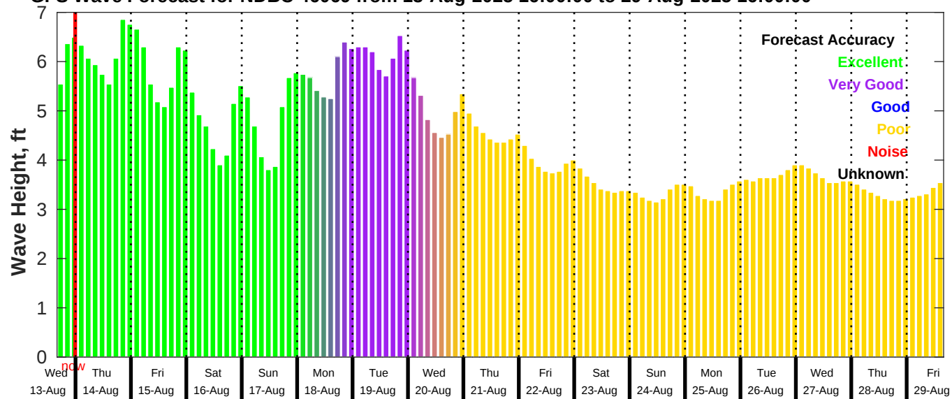
GFS Wave Forecast for NDBC 46069 from 13-Aug-2025 16:00:00 to 29-Aug-2025 16:00:00
