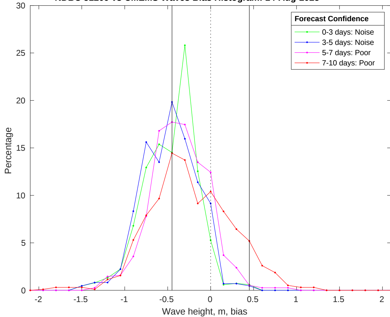
NDBC 51209 vs CMEMS Waves Bias Histogram: 14-Aug-2025
