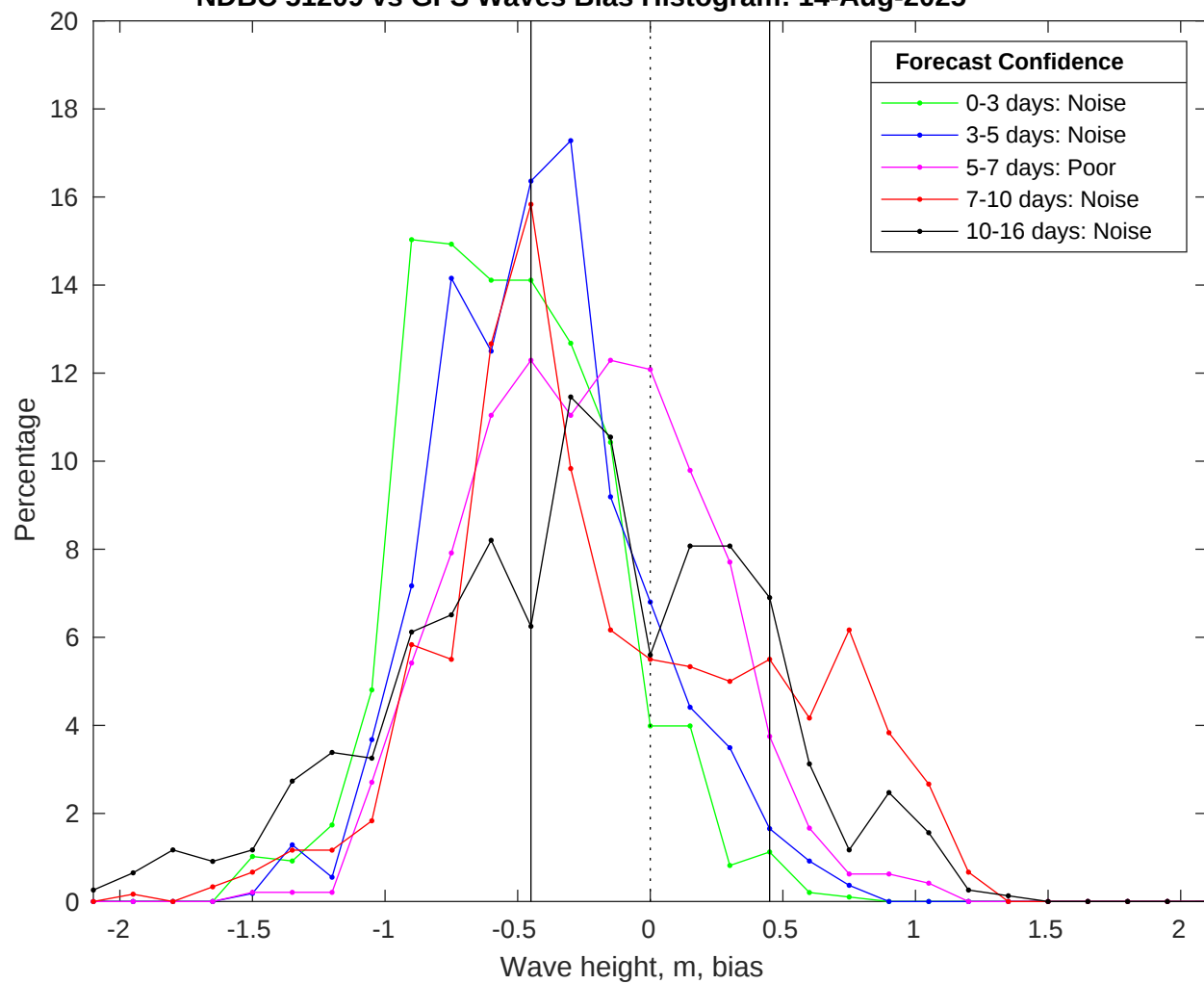
NDBC 51209 vs GFS Waves Bias Histogram: 14-Aug-2025
