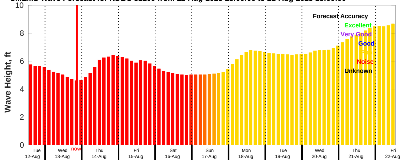
CMEMS Wave Forecast for NDBC 51209 from 12-Aug-2025 13:00:00 to 22-Aug-2025 13:00:00
