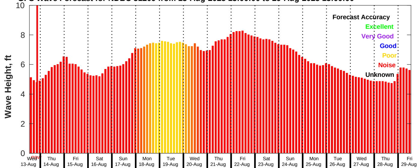
GFS Wave Forecast for NDBC 51209 from 13-Aug-2025 13:00:00 to 29-Aug-2025 13:00:00
