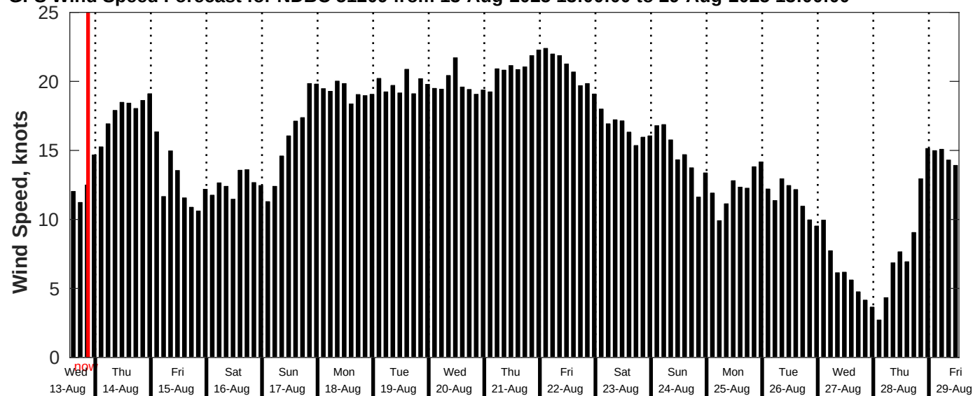
GFS Wind Speed Forecast for NDBC 51209 from 13-Aug-2025 13:00:00 to 29-Aug-2025 13:00:00
