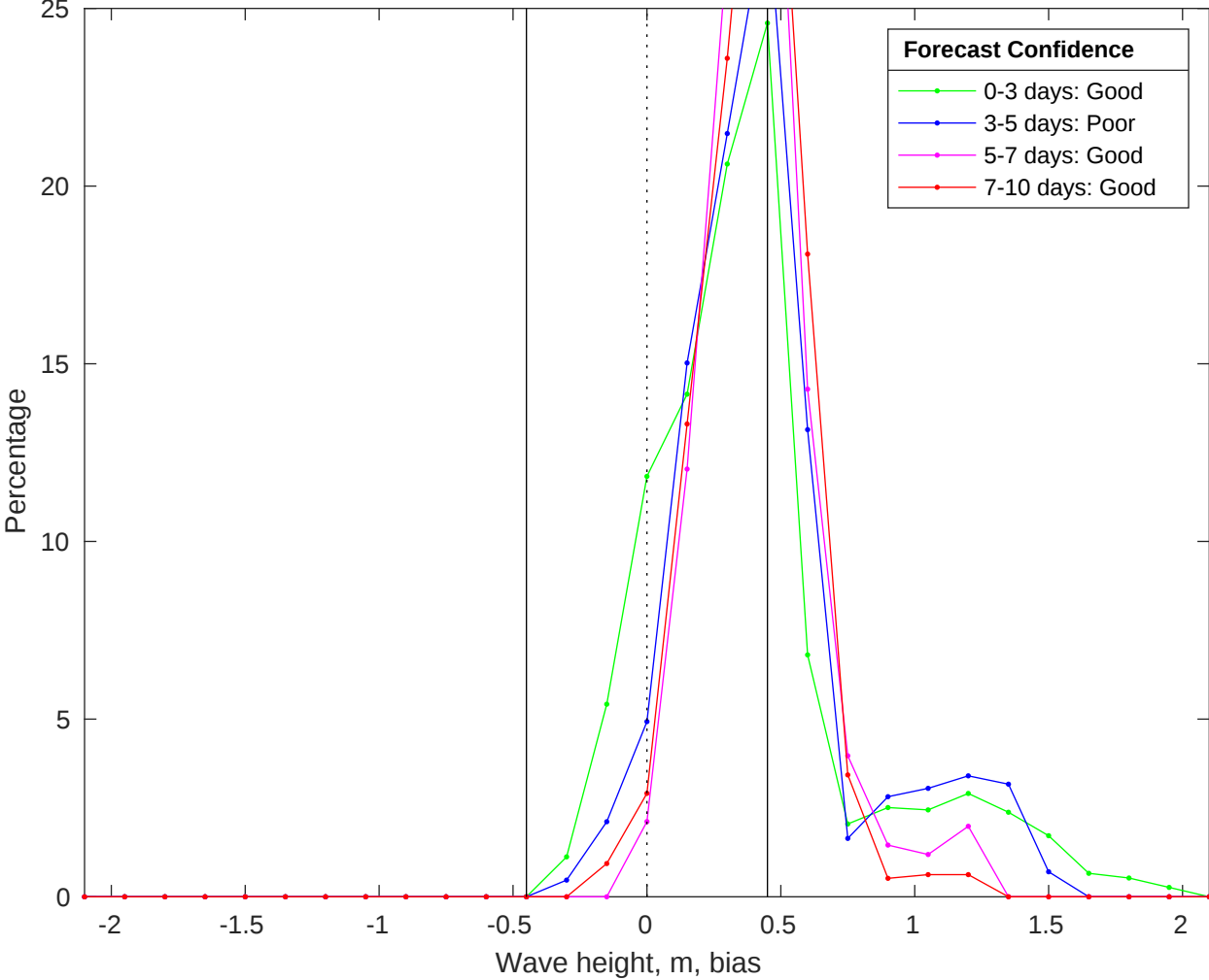
NDBC 51211 vs CMEMS Waves Bias Histogram: 14-Aug-2025
