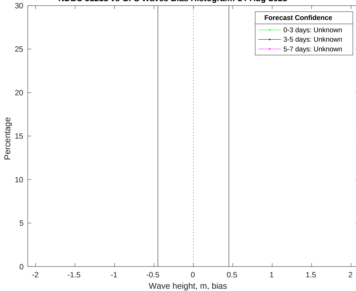
NDBC 51211 vs GFS Waves Bias Histogram: 14-Aug-2025
