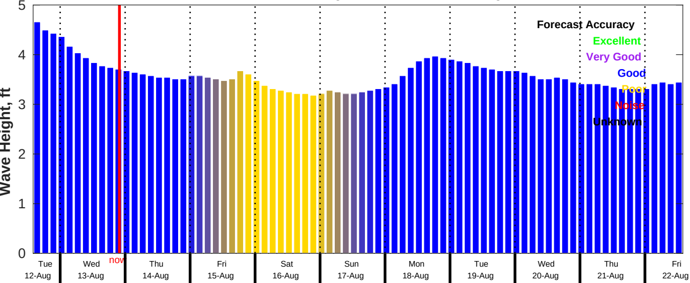
CMEMS Wave Forecast for NDBC 51211 from 12-Aug-2025 14:00:00 to 22-Aug-2025 14:00:00
