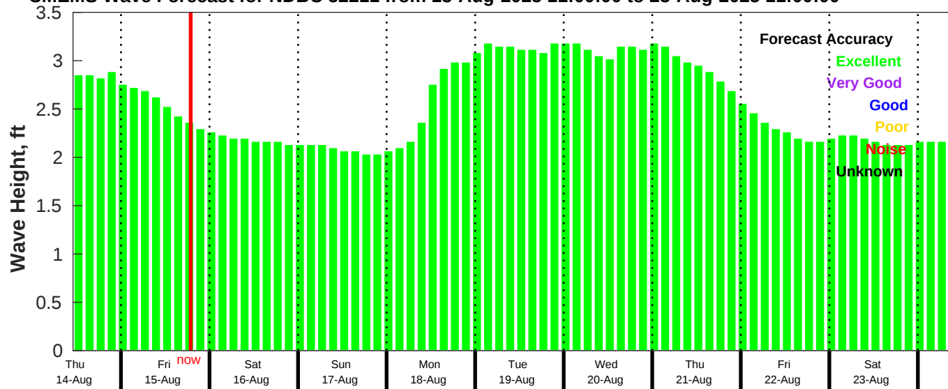
CMEMS Wave Forecast for NDBC 52211 from 13-Aug-2025 11:00:00 to 23-Aug-2025 11:00:00
