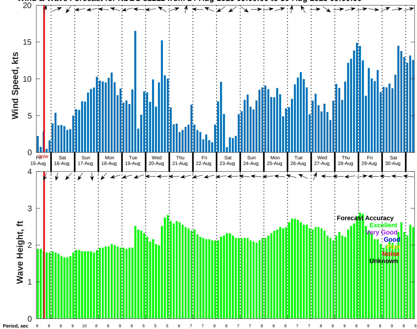
Wind & Wave Forecast for NDBC 52212 from 14-Aug-2025 09:00:00 to 30-Aug-2025 09:00:00
