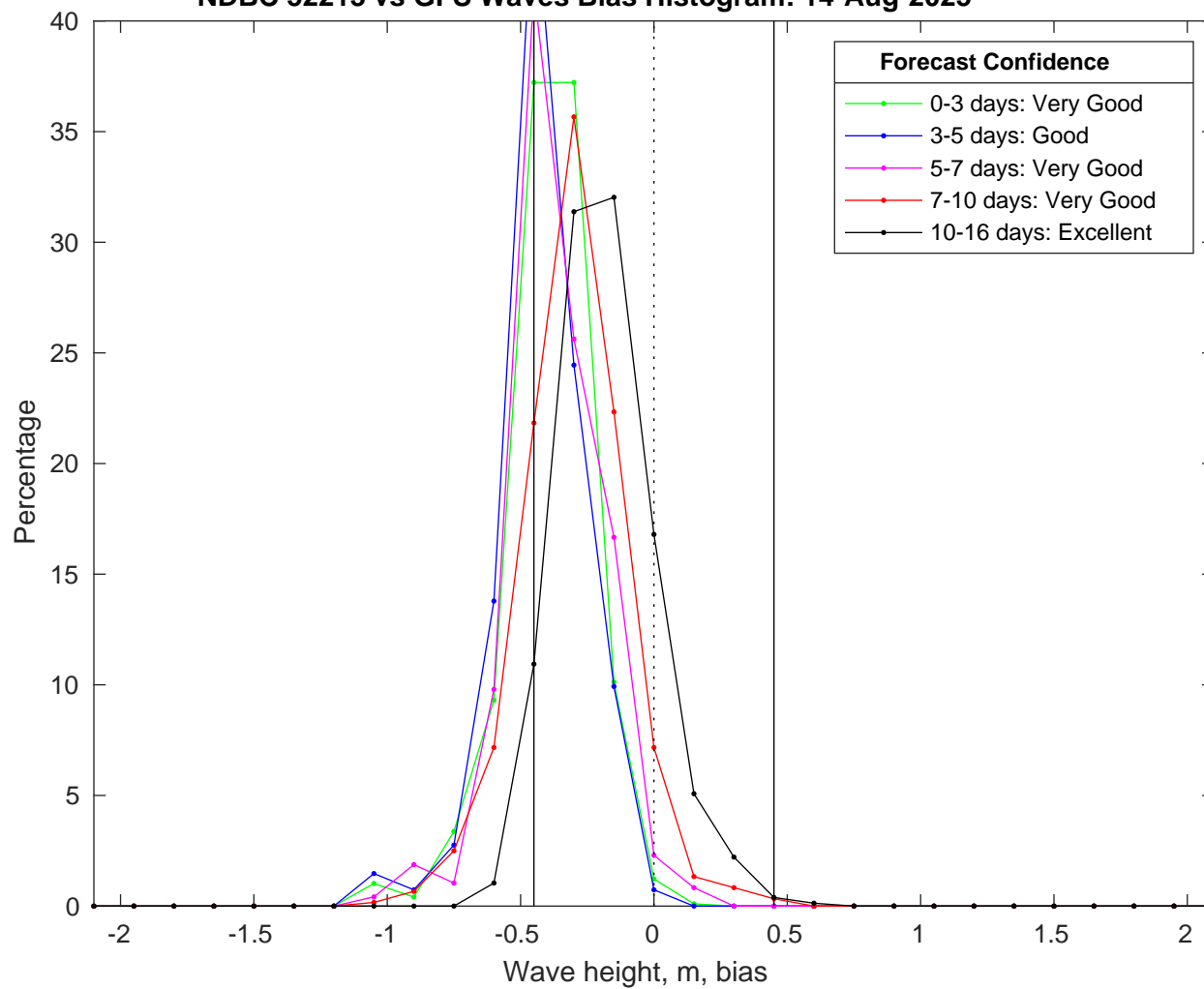
NDBC 52213 vs GFS Waves Bias Histogram: 14-Aug-2025
