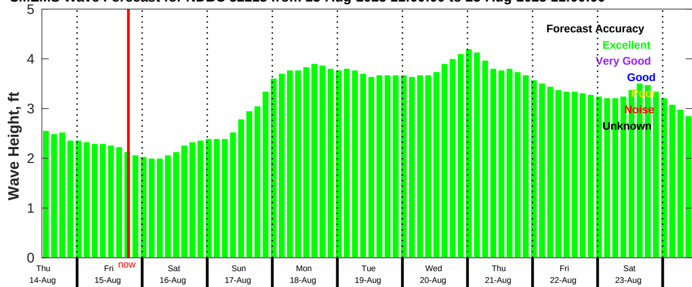
CMEMS Wave Forecast for NDBC 52213 from 13-Aug-2025 11:00:00 to 23-Aug-2025 11:00:00
