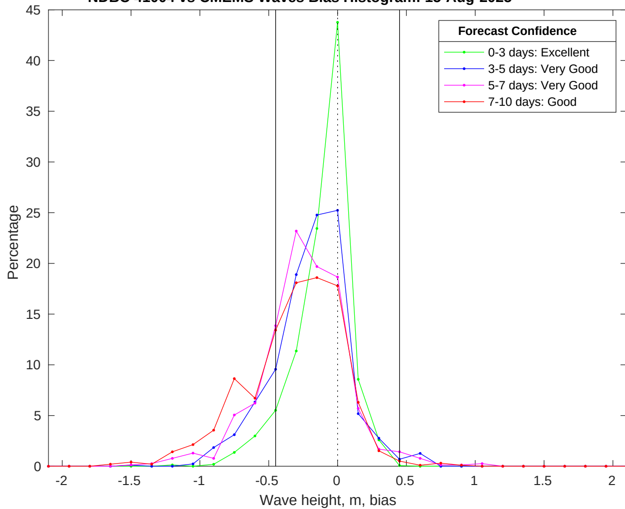
NDBC 41004 vs CMEMS Waves Bias Histogram: 15-Aug-2025
