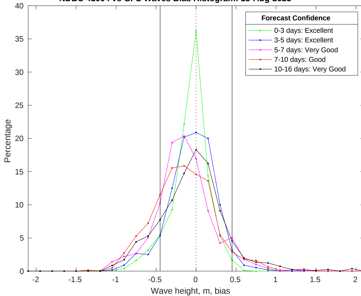
NDBC 41004 vs GFS Waves Bias Histogram: 15-Aug-2025
