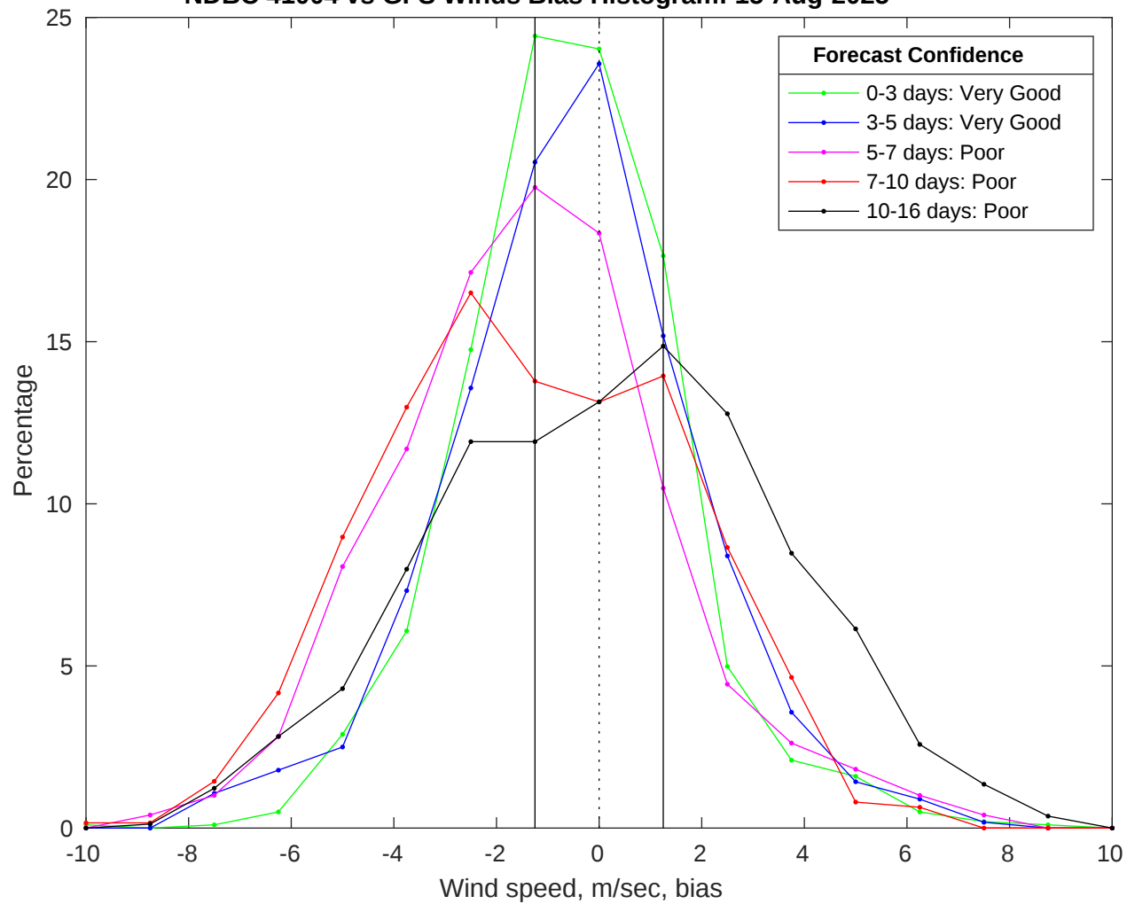
NDBC 41004 vs GFS Winds Bias Histogram: 15-Aug-2025
