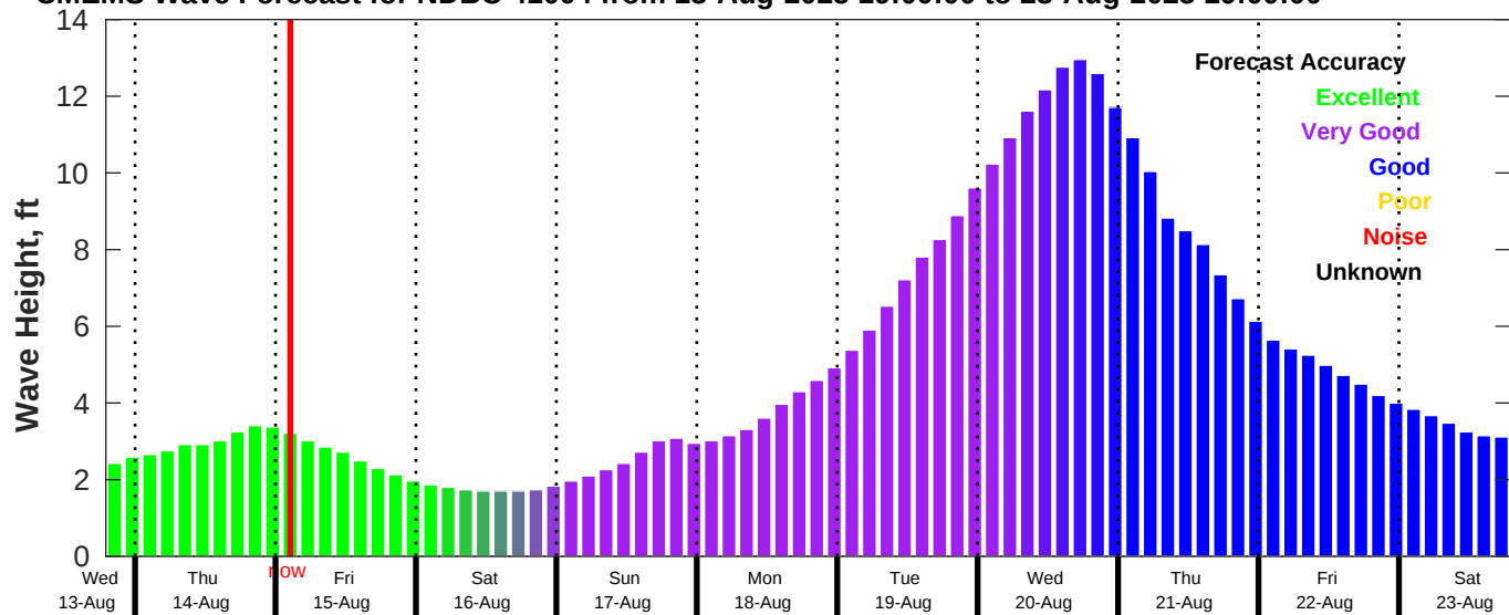
CMEMS Wave Forecast for NDBC 41004 from 13-Aug-2025 19:00:00 to 23-Aug-2025 19:00:00
