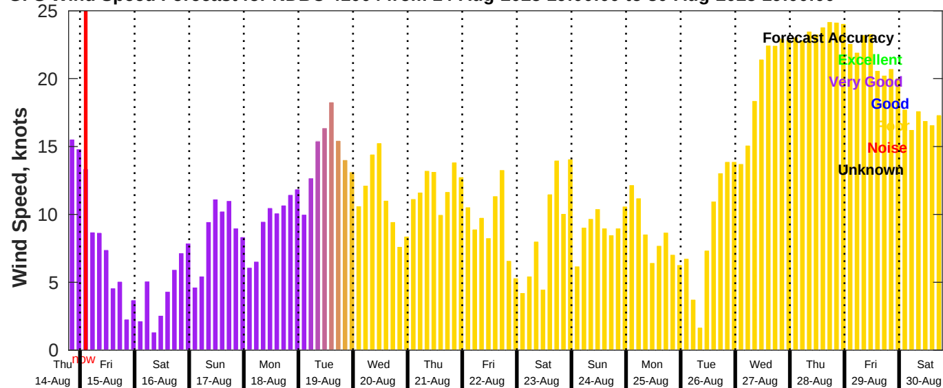
GFS Wind Speed Forecast for NDBC 41004 from 14-Aug-2025 19:00:00 to 30-Aug-2025 19:00:00
