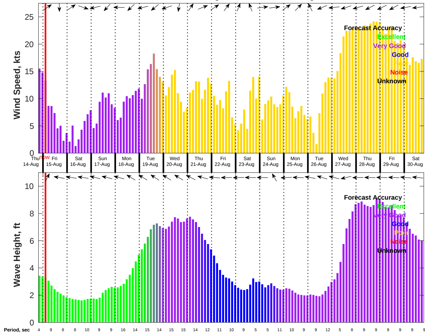
Wind & Wave Forecast for NDBC 41004 from 14-Aug-2025 19:00:00 to 30-Aug-2025 19:00:00
