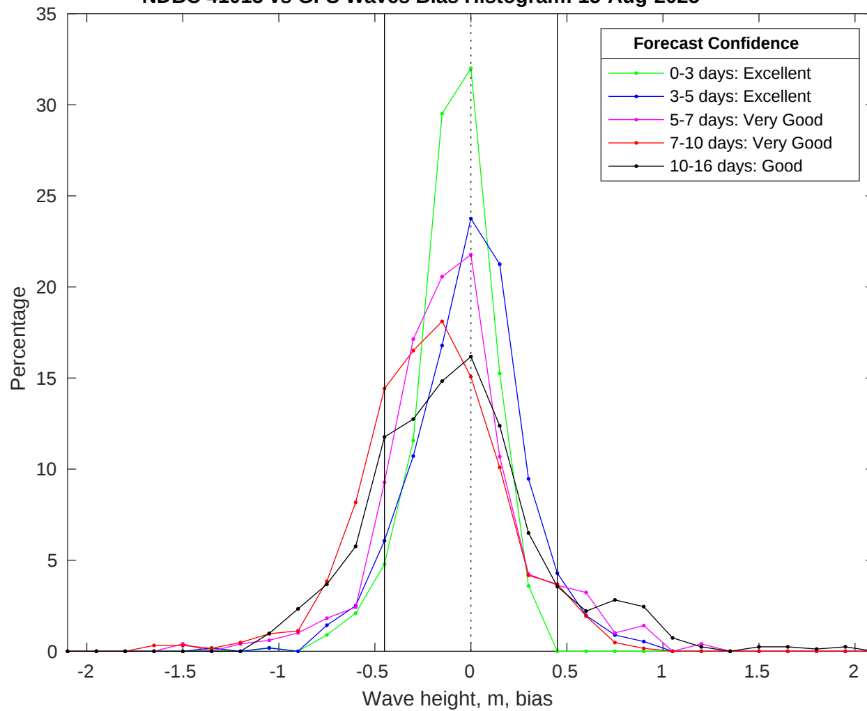
NDBC 41013 vs GFS Waves Bias Histogram: 15-Aug-2025
