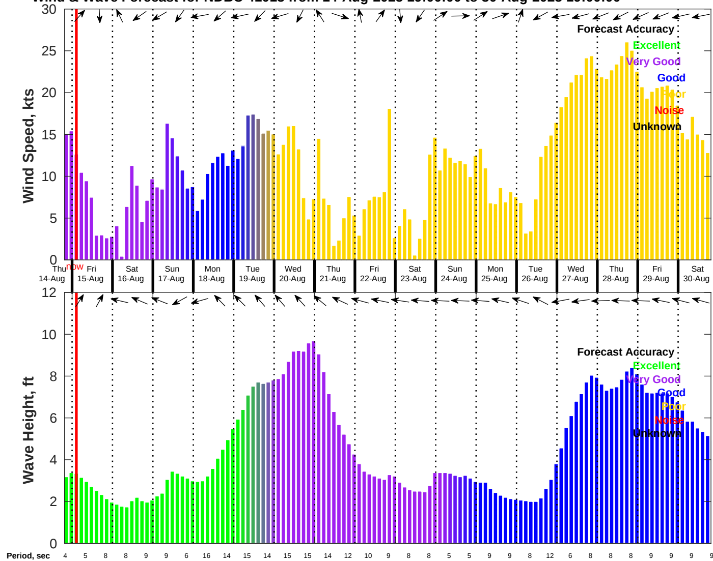
Wind & Wave Forecast for NDBC 41013 from 14-Aug-2025 19:00:00 to 30-Aug-2025 19:00:00
