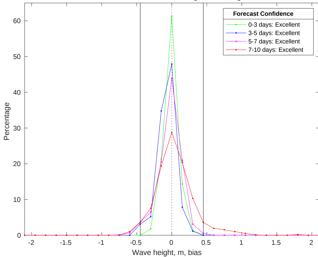
NDBC 41040 vs CMEMS Waves Bias Histogram: 15-Aug-2025
