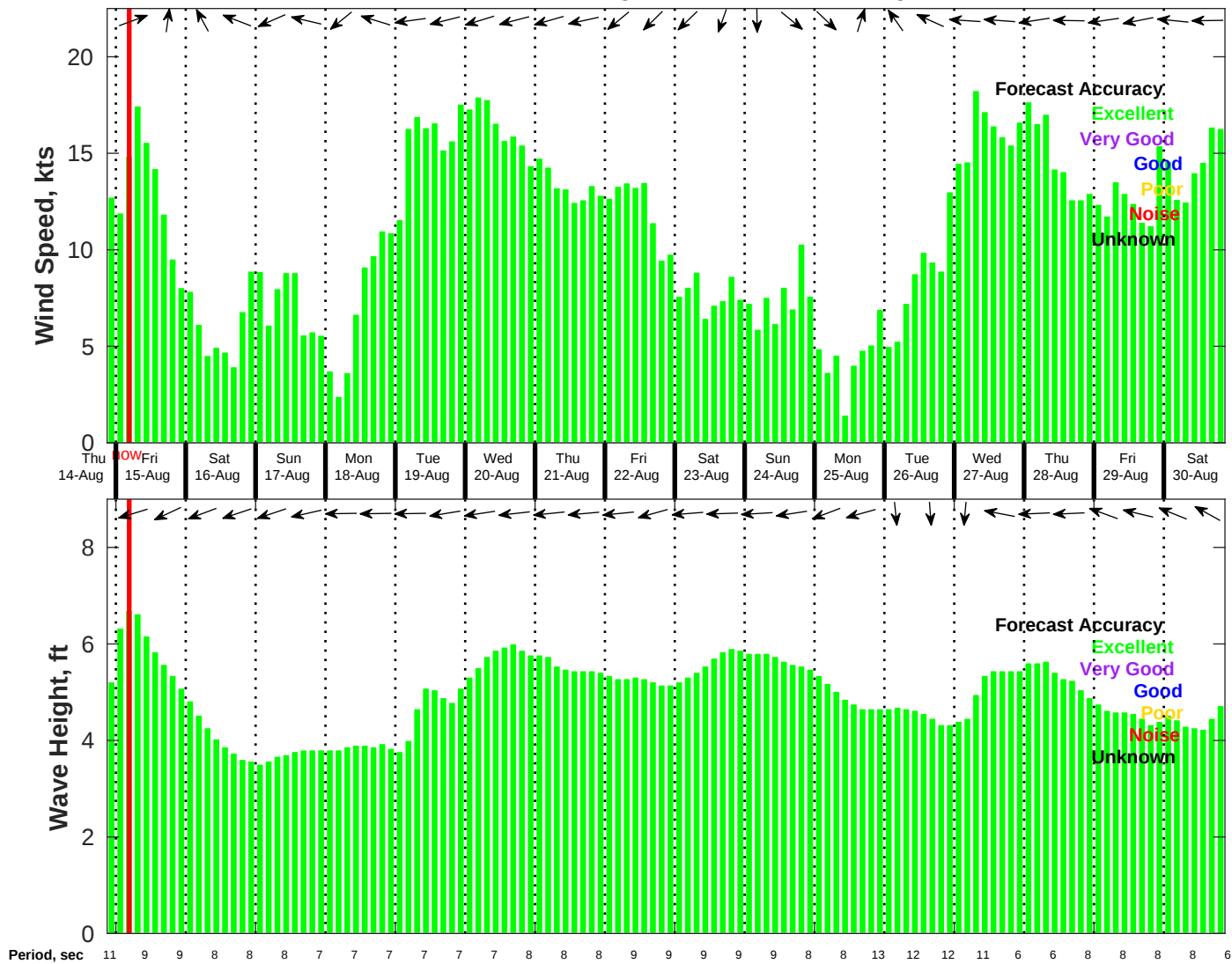
Wind & Wave Forecast for NDBC 41040 from 14-Aug-2025 21:00:00 to 30-Aug-2025 21:00:00
