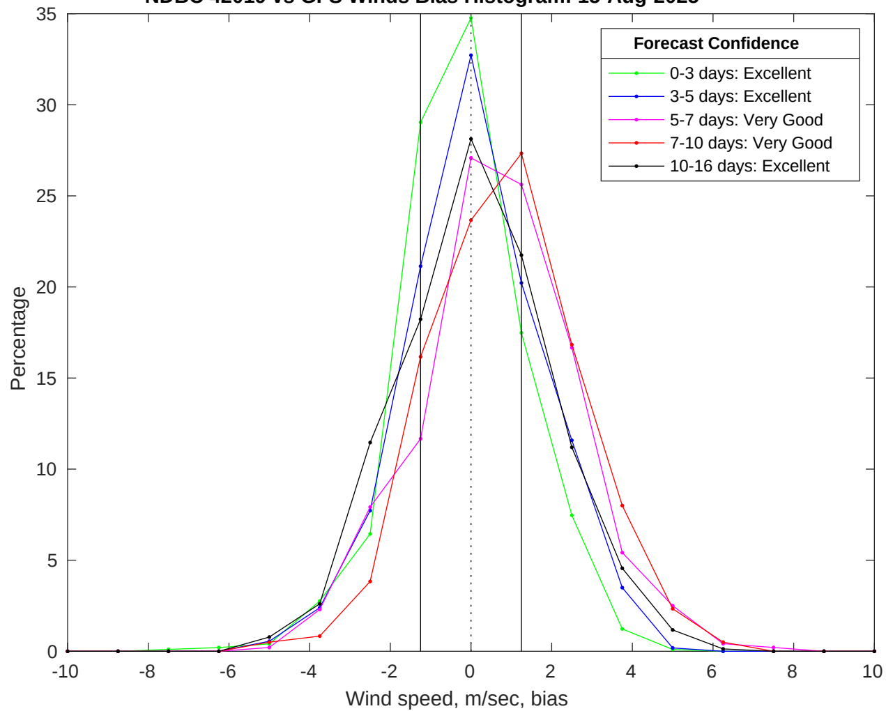
NDBC 42019 vs GFS Winds Bias Histogram: 15-Aug-2025
