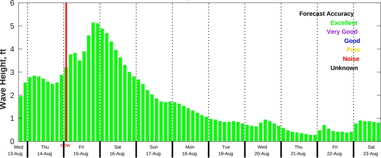
CMEMS Wave Forecast for NDBC 42019 from 13-Aug-2025 18:00:00 to 23-Aug-2025 18:00:00
