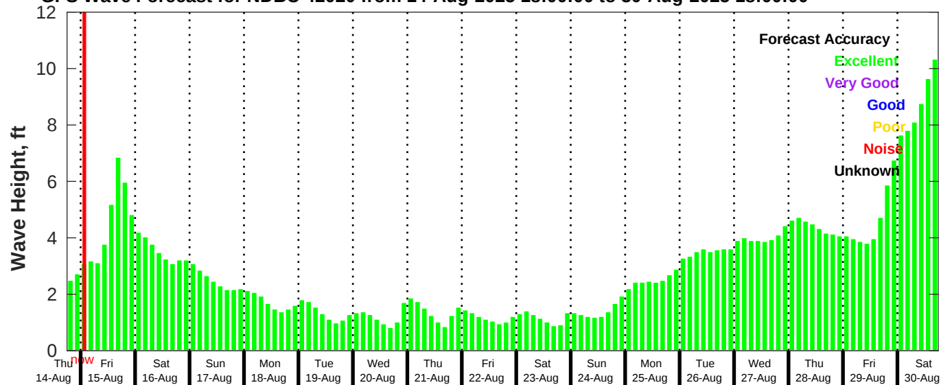
GFS Wave Forecast for NDBC 42020 from 14-Aug-2025 18:00:00 to 30-Aug-2025 18:00:00
