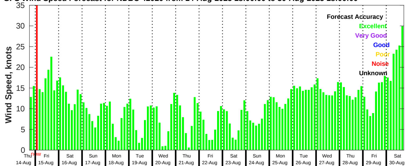
GFS Wind Speed Forecast for NDBC 42020 from 14-Aug-2025 18:00:00 to 30-Aug-2025 18:00:00
