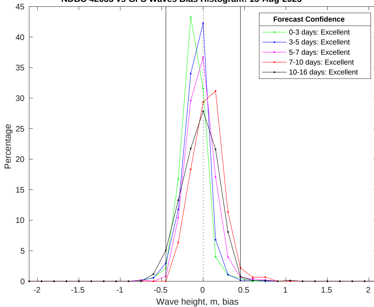
NDBC 42035 vs GFS Waves Bias Histogram: 15-Aug-2025
