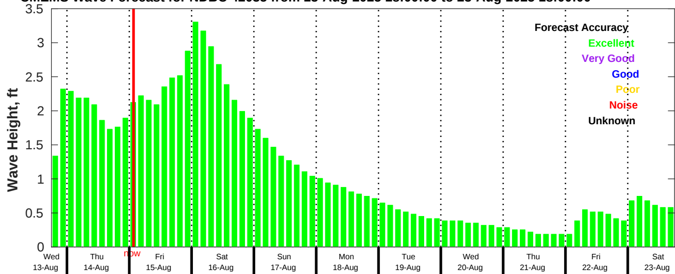
CMEMS Wave Forecast for NDBC 42035 from 13-Aug-2025 18:00:00 to 23-Aug-2025 18:00:00
