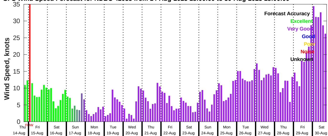
GFS Wind Speed Forecast for NDBC 42035 from 14-Aug-2025 18:00:00 to 30-Aug-2025 18:00:00
