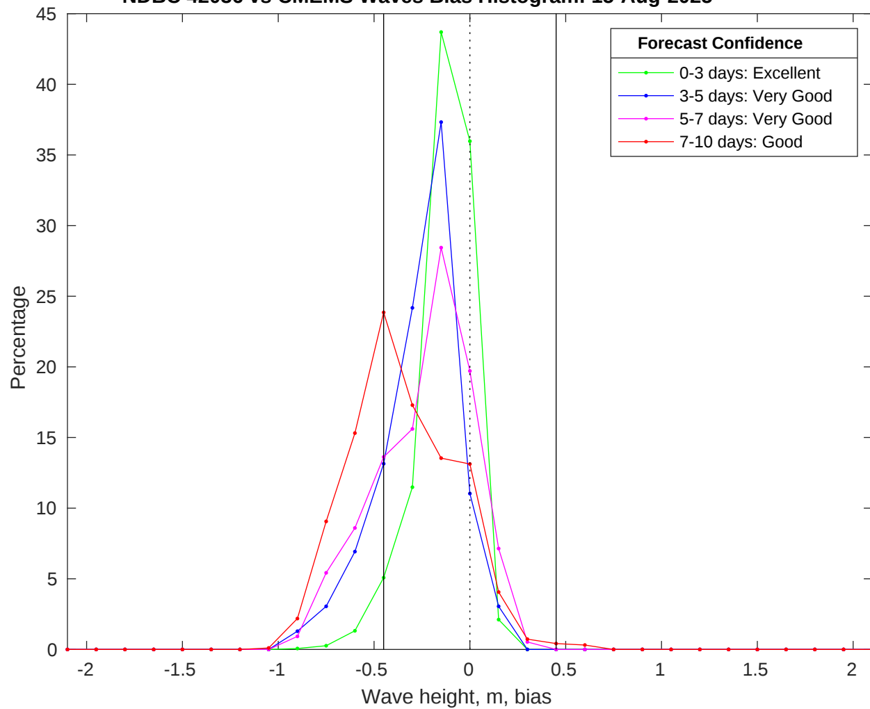
NDBC 42036 vs CMEMS Waves Bias Histogram: 15-Aug-2025
