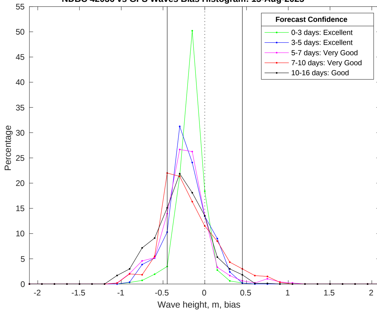
NDBC 42036 vs GFS Waves Bias Histogram: 15-Aug-2025
