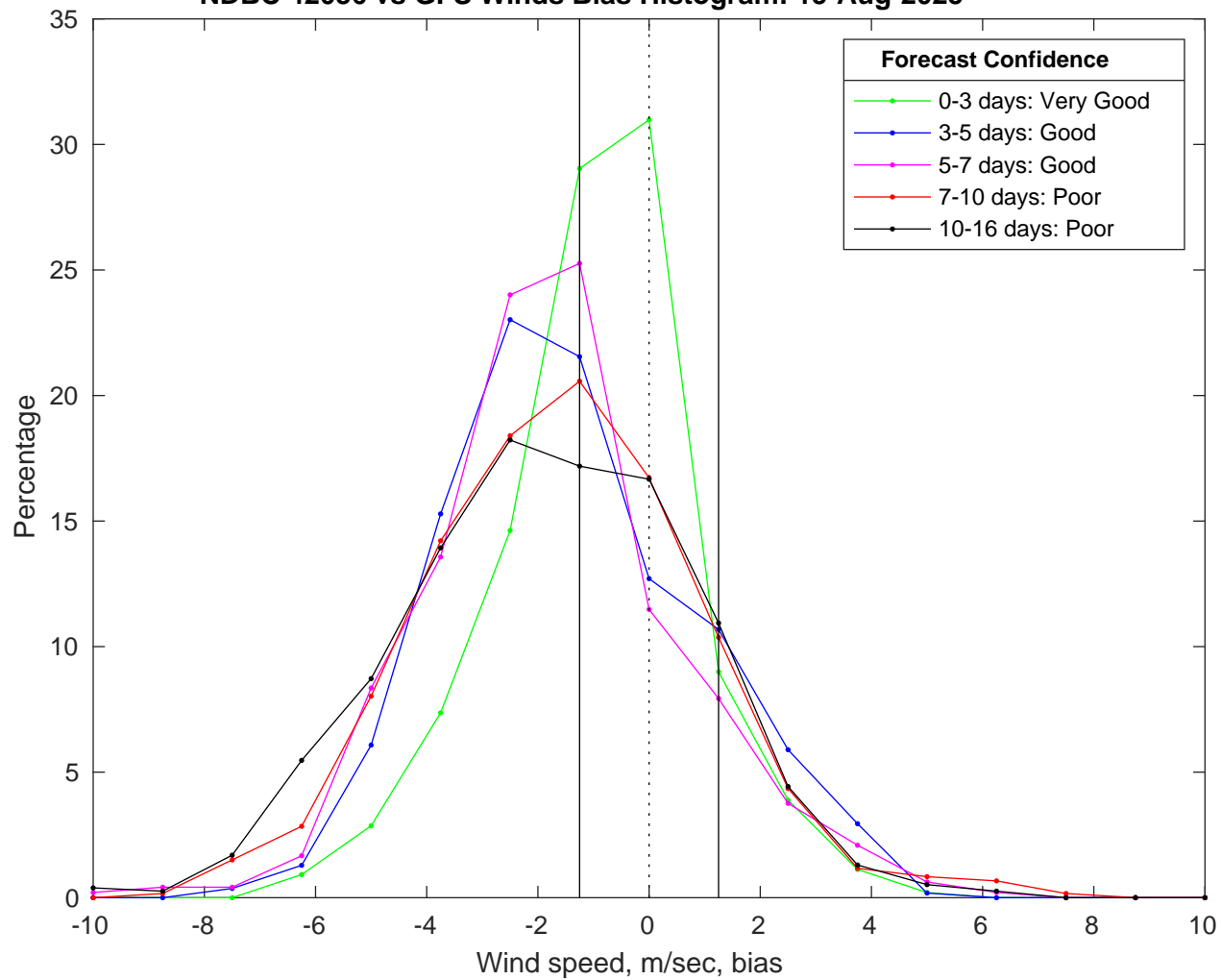
NDBC 42036 vs GFS Winds Bias Histogram: 15-Aug-2025
