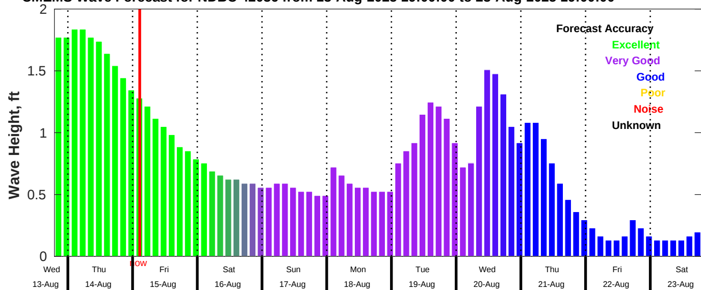
CMEMS Wave Forecast for NDBC 42036 from 13-Aug-2025 19:00:00 to 23-Aug-2025 19:00:00
