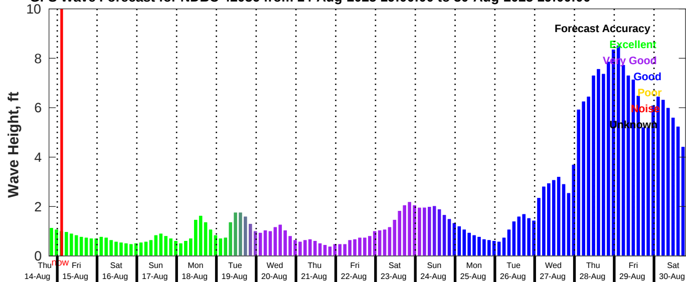
GFS Wave Forecast for NDBC 42036 from 14-Aug-2025 19:00:00 to 30-Aug-2025 19:00:00
