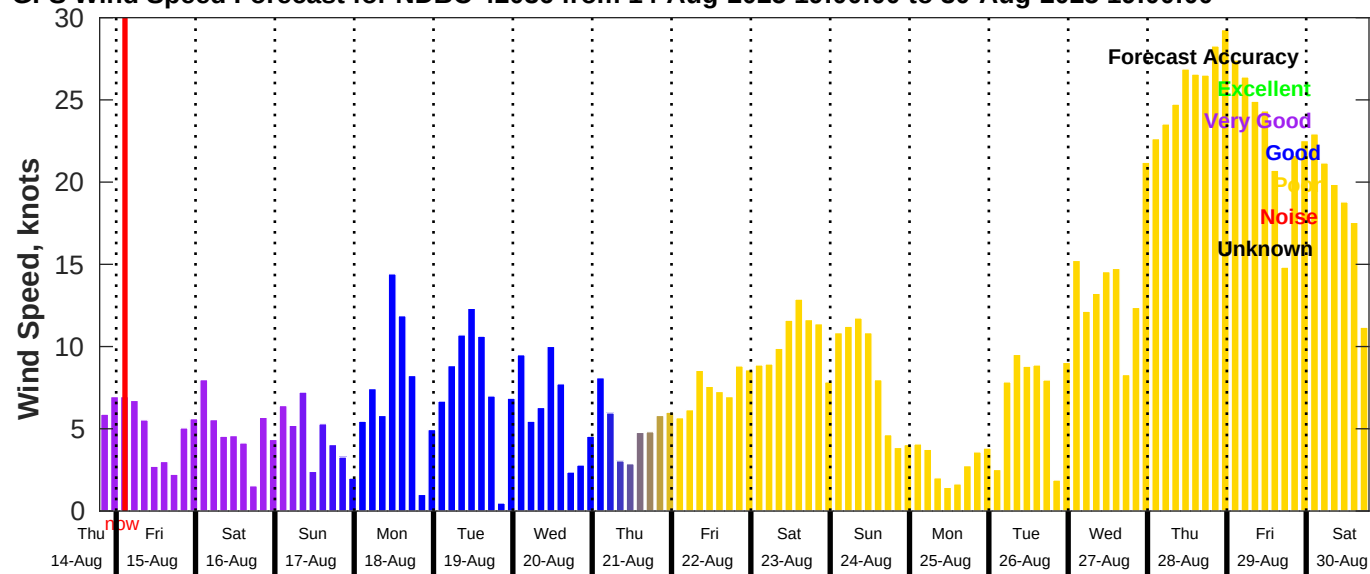
GFS Wind Speed Forecast for NDBC 42036 from 14-Aug-2025 19:00:00 to 30-Aug-2025 19:00:00
