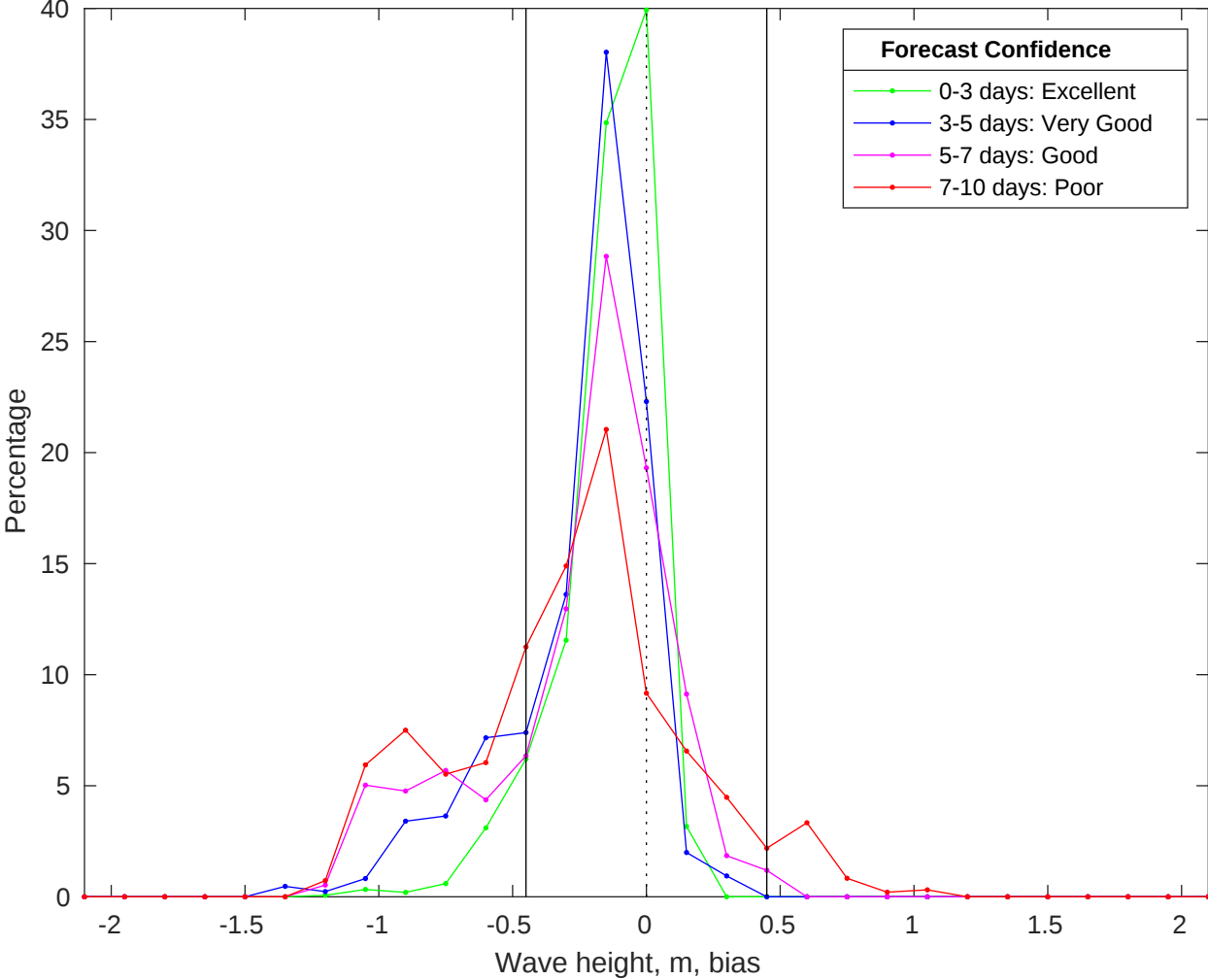
NDBC 42040 vs CMEMS Waves Bias Histogram: 15-Aug-2025
