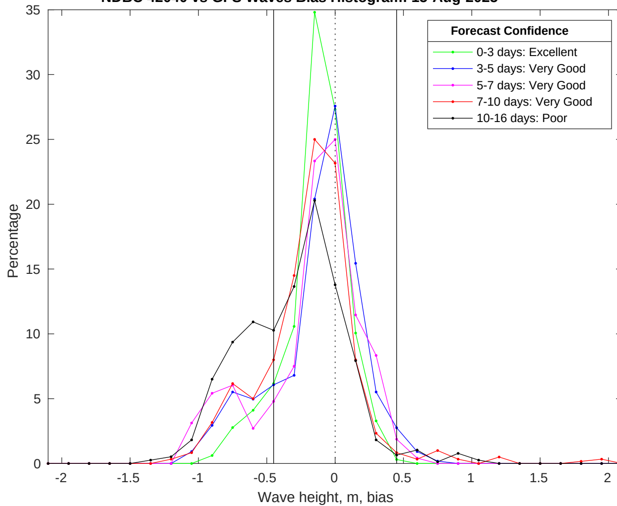
NDBC 42040 vs GFS Waves Bias Histogram: 15-Aug-2025
