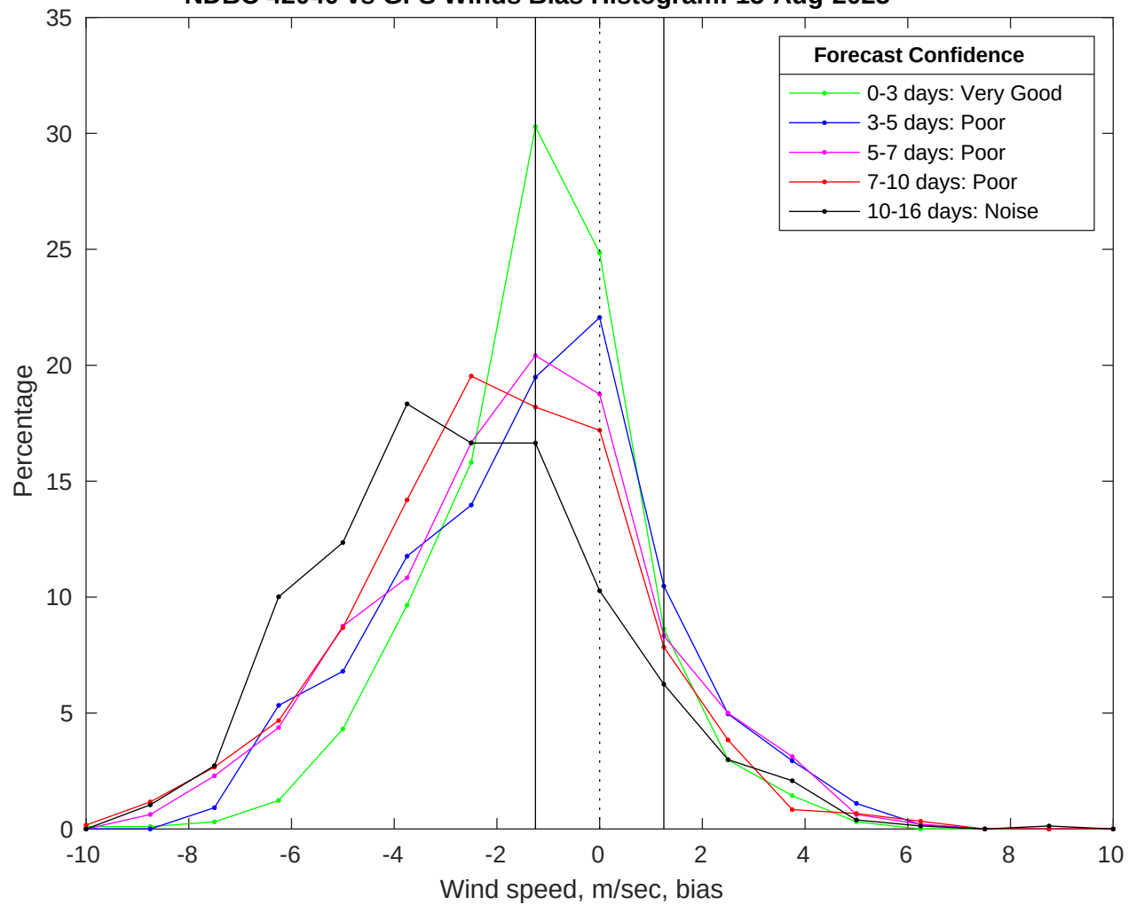
NDBC 42040 vs GFS Winds Bias Histogram: 15-Aug-2025
