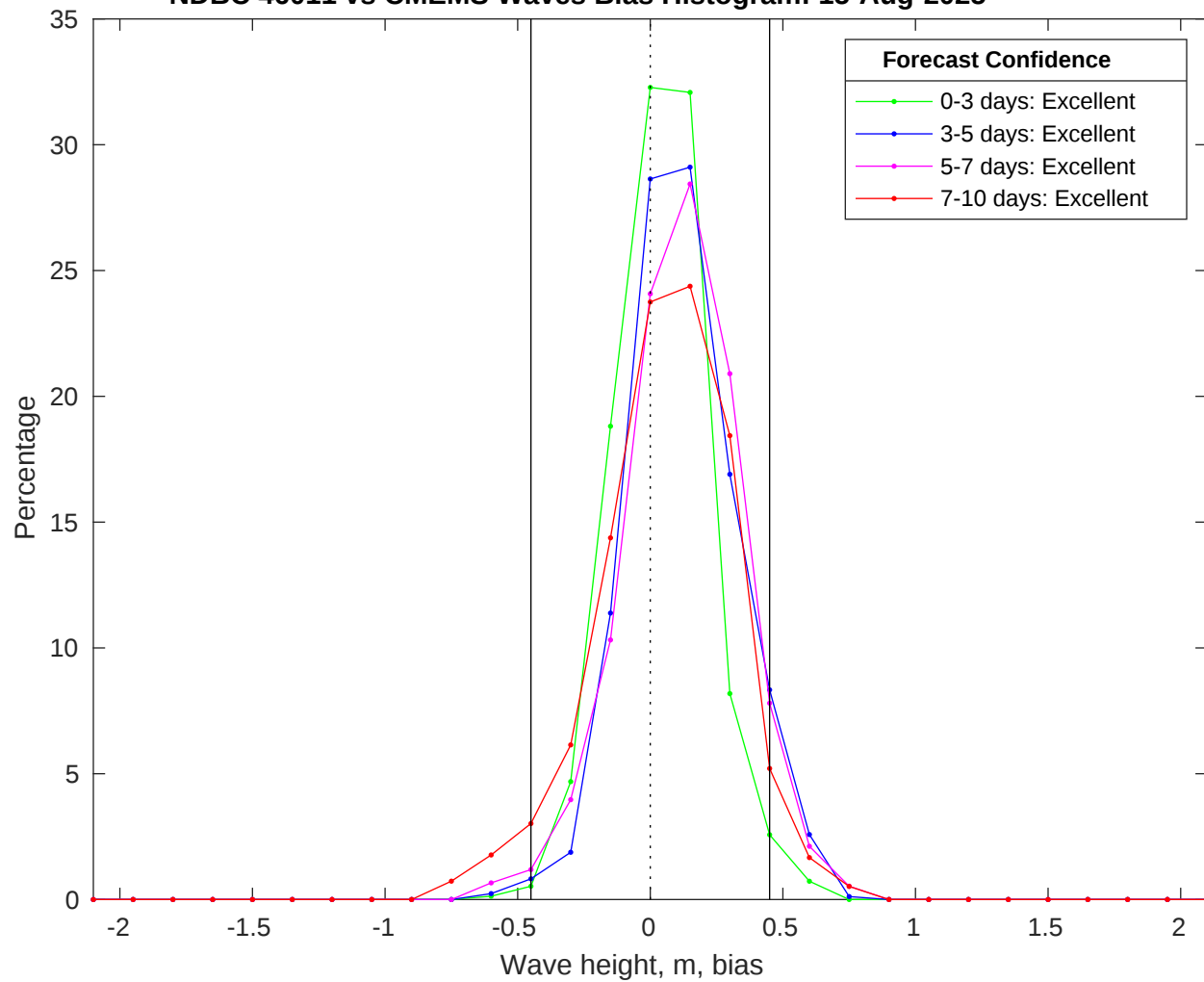
NDBC 46011 vs CMEMS Waves Bias Histogram: 15-Aug-2025
