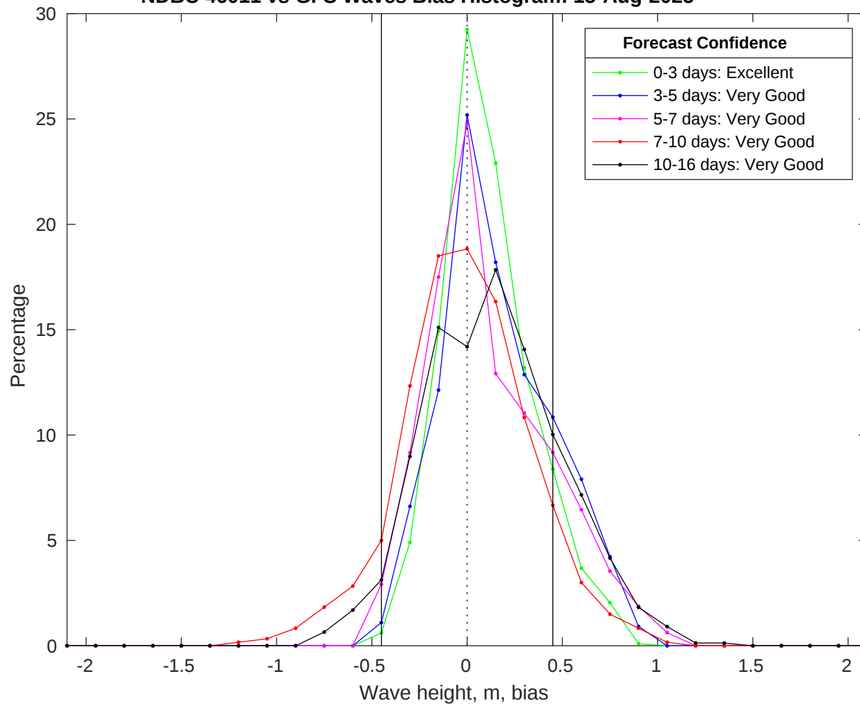
NDBC 46011 vs GFS Waves Bias Histogram: 15-Aug-2025
