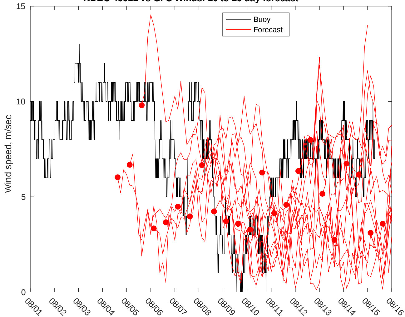
NDBC 46011 vs GFS Winds: 10 to 16 day forecast
