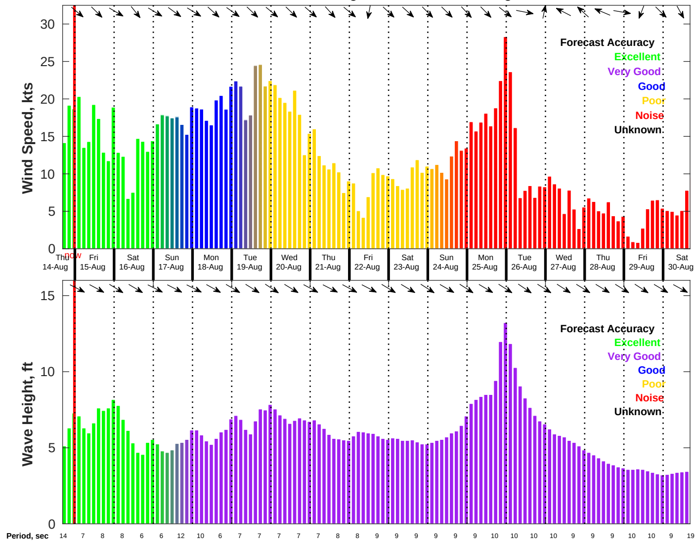
Wind & Wave Forecast for NDBC 46011 from 14-Aug-2025 16:00:00 to 30-Aug-2025 16:00:00
