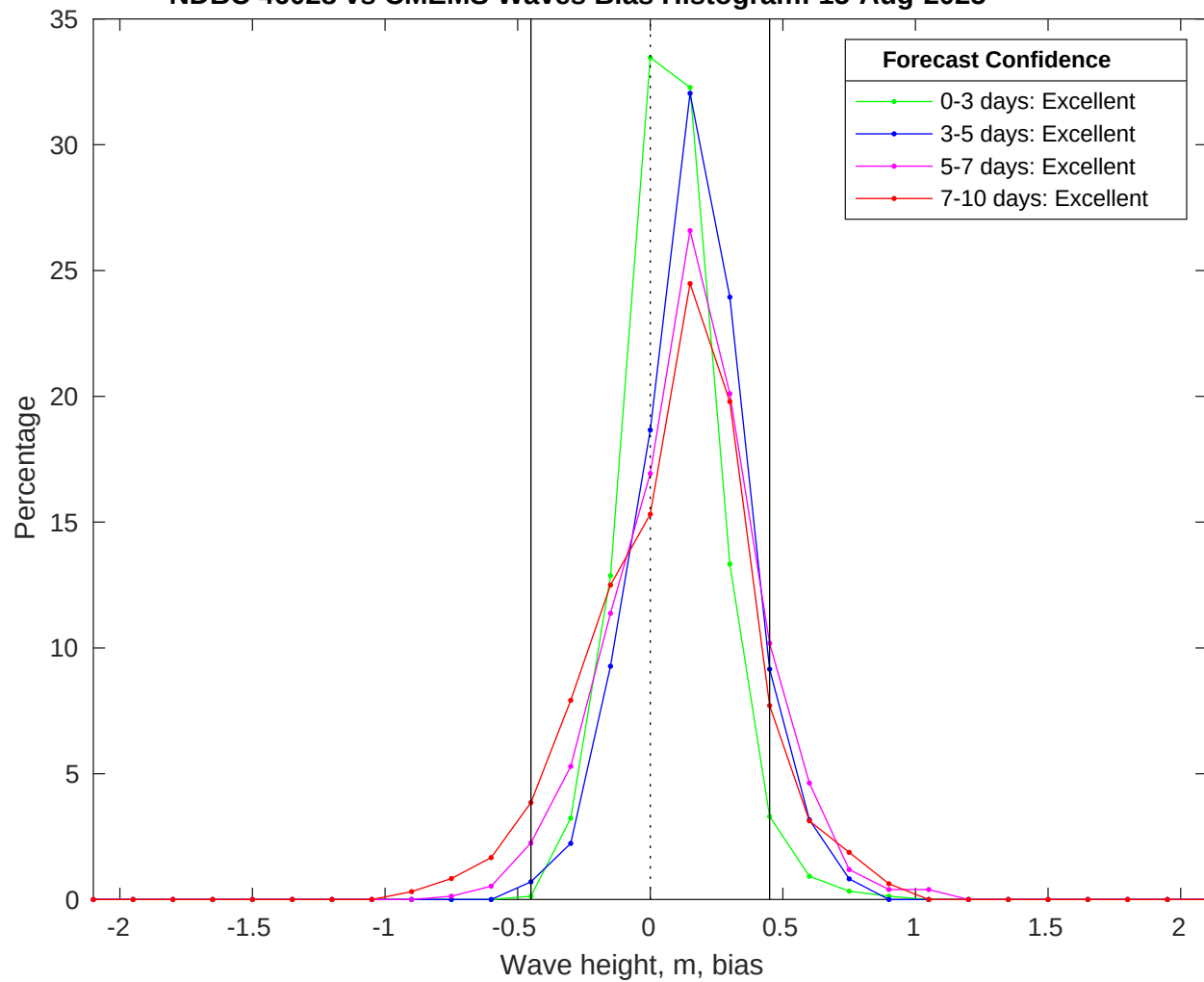
NDBC 46028 vs CMEMS Waves Bias Histogram: 15-Aug-2025
