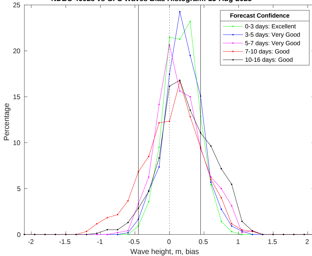
NDBC 46028 vs GFS Waves Bias Histogram: 15-Aug-2025
