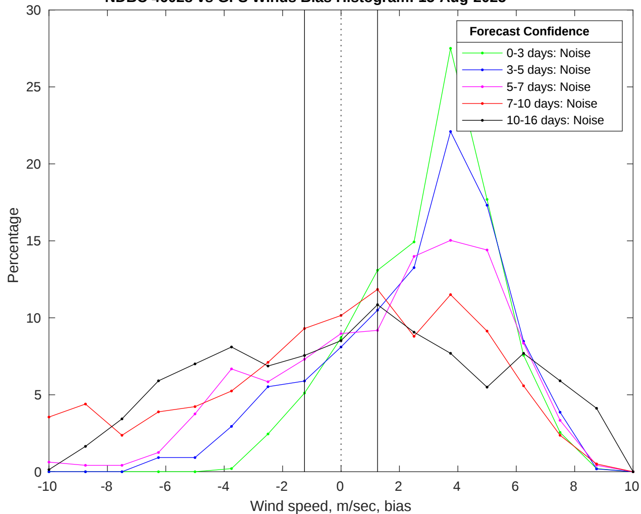
NDBC 46028 vs GFS Winds Bias Histogram: 15-Aug-2025
