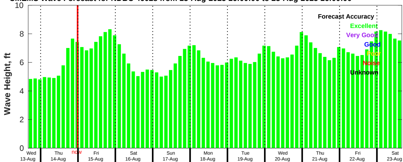
CMEMS Wave Forecast for NDBC 46028 from 13-Aug-2025 16:00:00 to 23-Aug-2025 16:00:00
